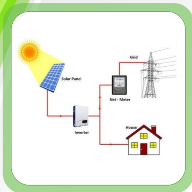
On-Grid System
